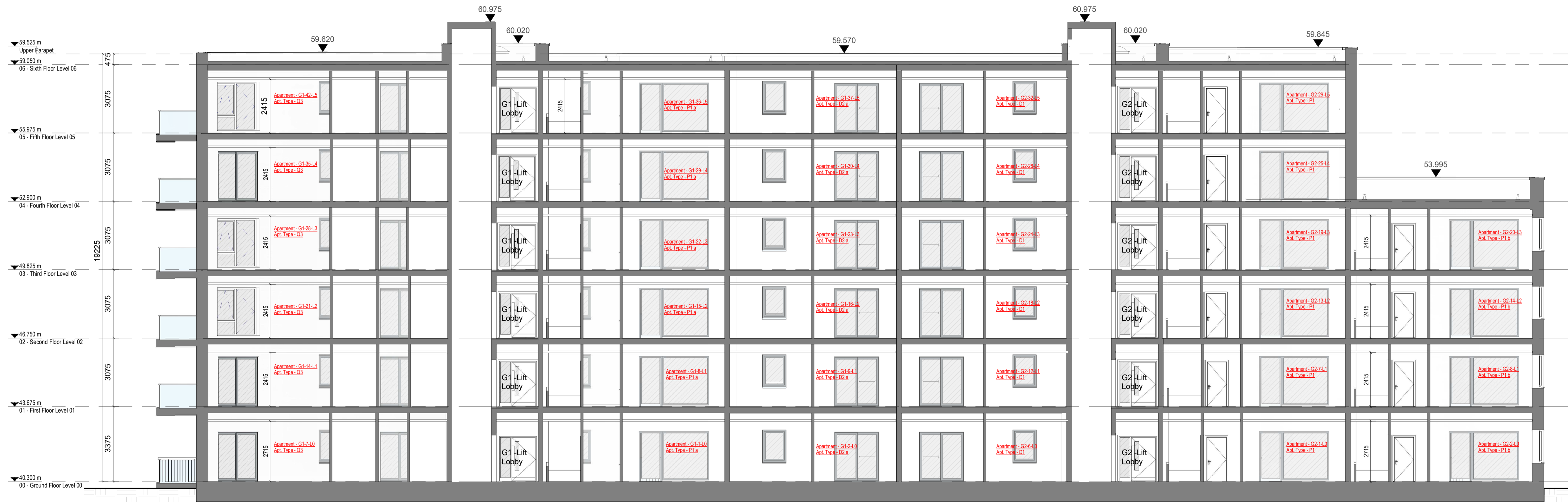
1 GA - Section AA
